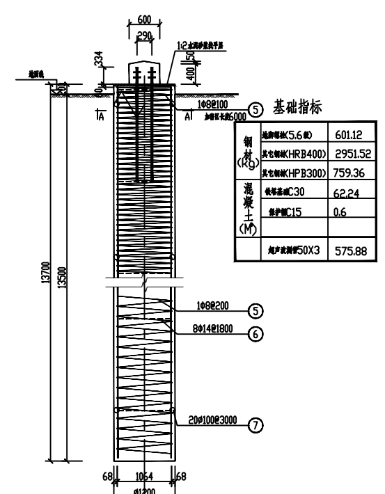
35-CD22S-J4灌注桩基础
