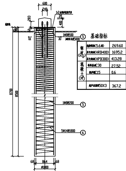
35-CD22D-J4灌注桩基础
